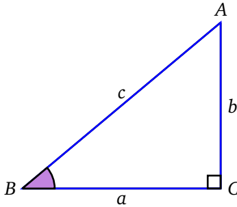
FIGURE 47.1: Mnemonic for the sin trigonometric function. For the angle B , the opposite side is b and the hypotenuse is c and \sin B = \frac{b}{c} . The first letters of each word in the son of Hamlet mnemonic are s , o , and h , corresponding respectively to sine , opposite and hypotenuse .
